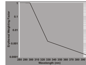
Erythral Action Spectrum Source: The International Commission on Illumination
